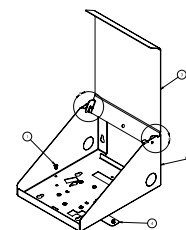
Part# LMWWU12127 Clamshell mount
