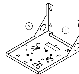
Part# LBWWU975 Right angle wall mount
