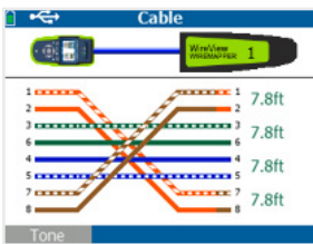
Cable wiring validation
