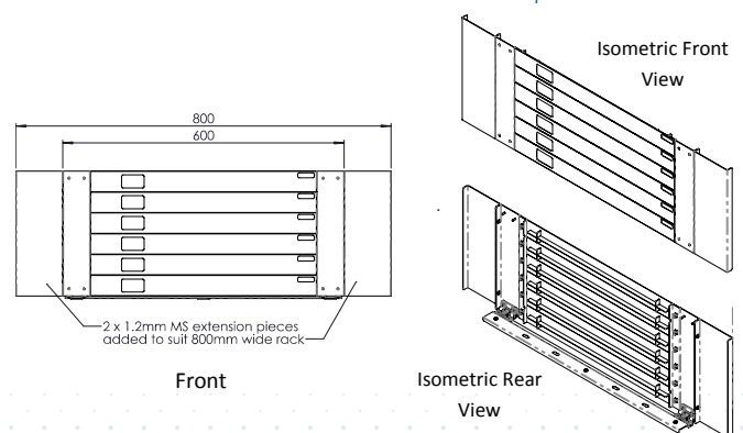
Bracket with 100mm panel extensions
