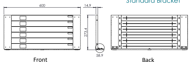
Standard Bracket
