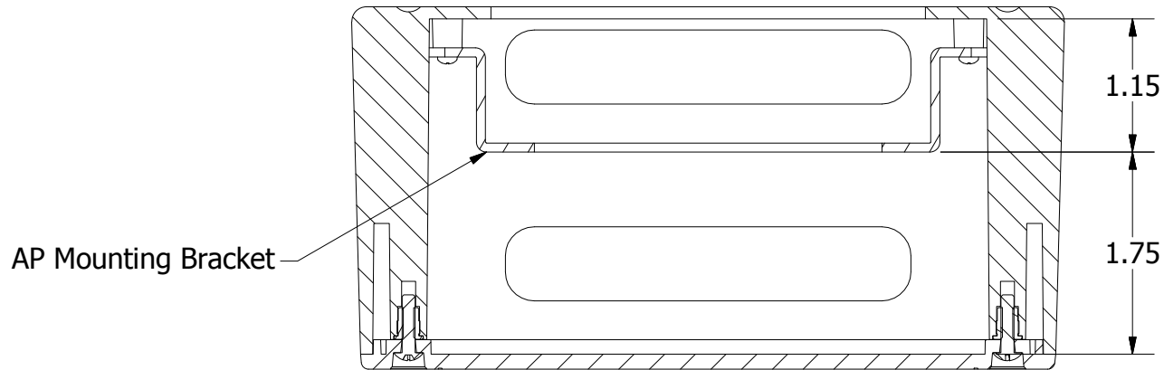
SECTION C-C SCALE 1 / 1.5
