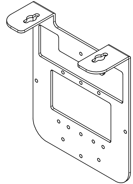
ISOMETRIC VIEW
