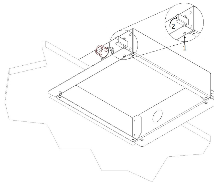
Figure 4 - Back Box Mounting
