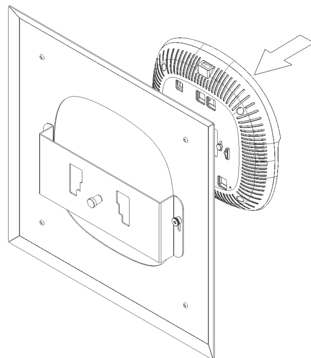
Figure 2 - Install Access Point
