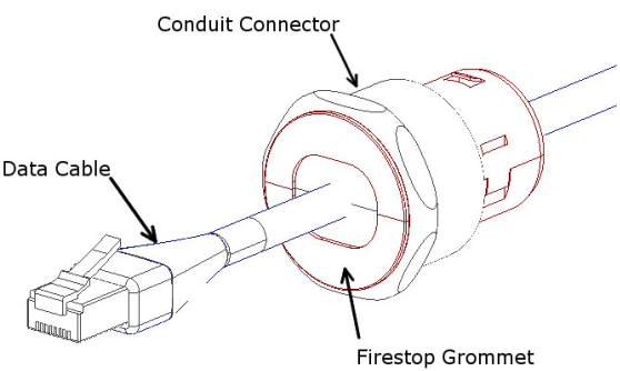
Figure 4 – Firestop Grommet
