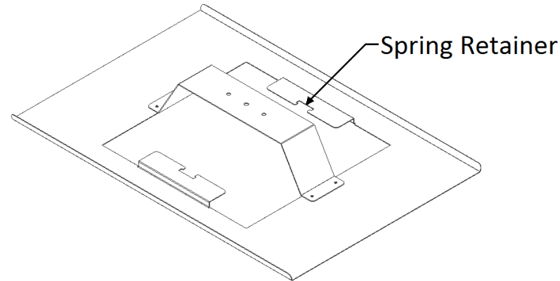
Figure 1 - Spring Retainer
