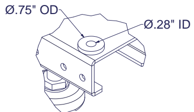
ASSOCIATED SHOULDER WASHER FOR SPLIT MESH DOOR
