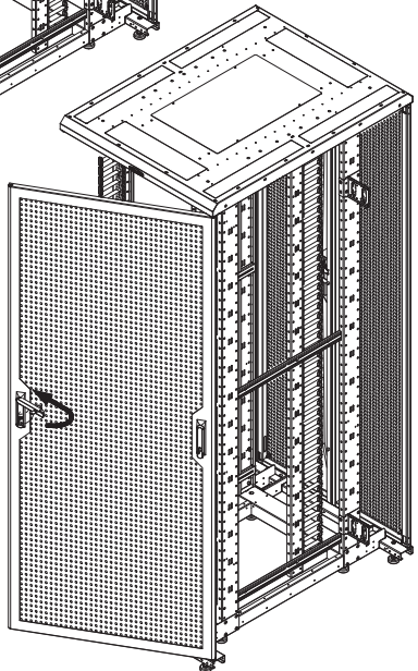
Door Opened with left handle; right handle completely latched closed
