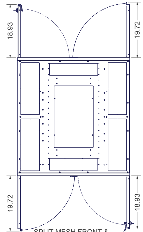
SPLIT MESH FRONT & REAR DOORS, PART #8402EN40SM TOP VIEW
