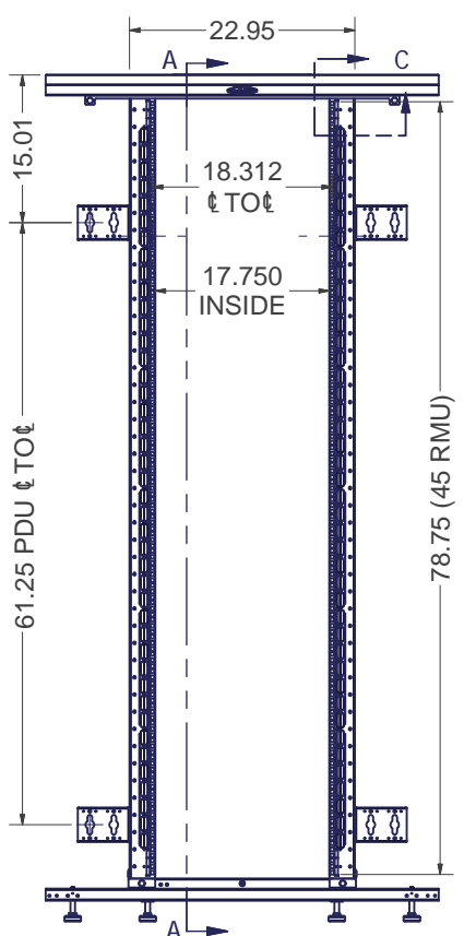
FRONT VIEW DOORS REMOVED
