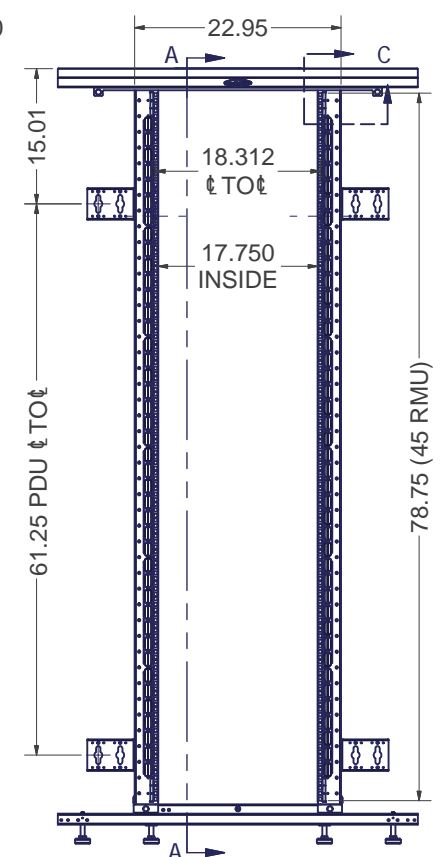
FRONT VIEW DOORS AND SIDES REMOVED
