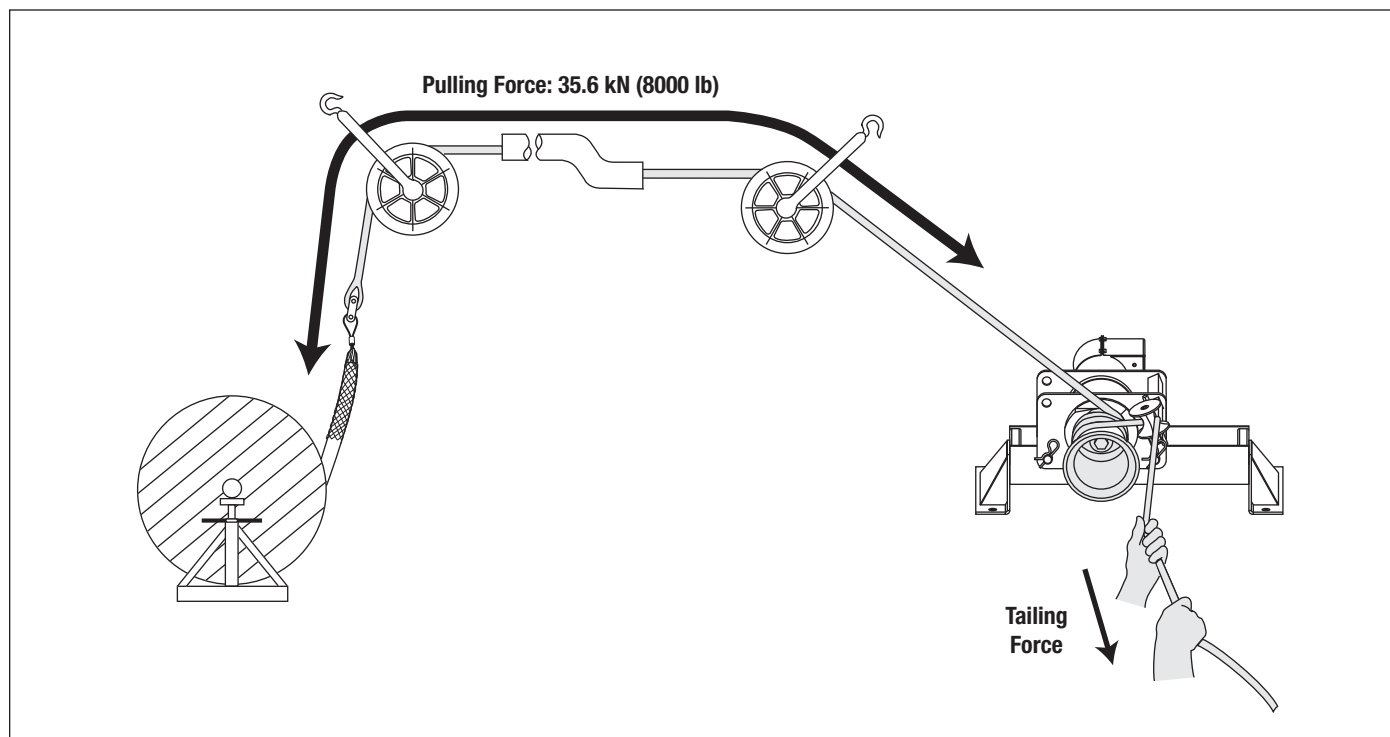
The Capstan as a Force Multiplier
