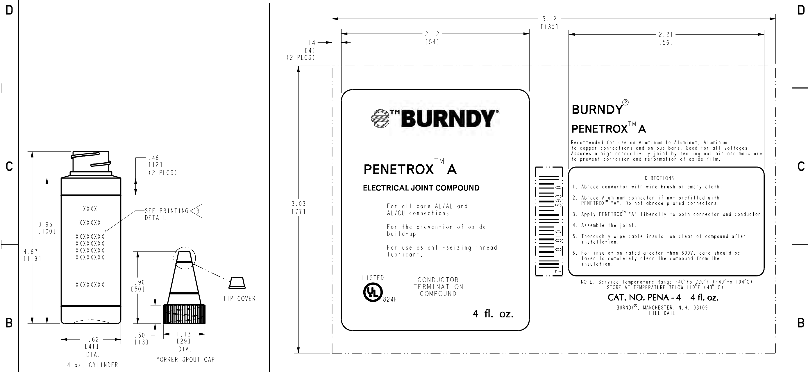
ENLARGED VIEW OF PRINTING DETAIL
