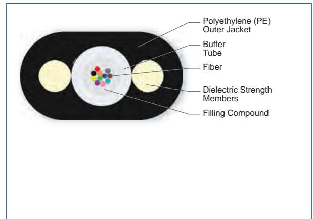
Cross Section of Part Number: 012EBZ-14101A20
