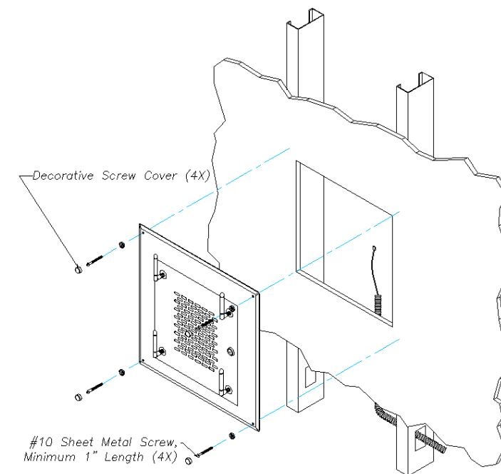
Figure 4 - Wall installation.
