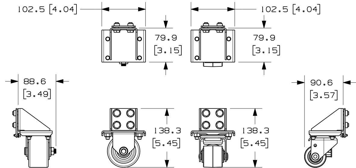
FIXED CASTER
