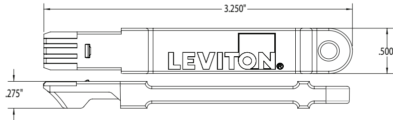
EXTRACTION TOOL
