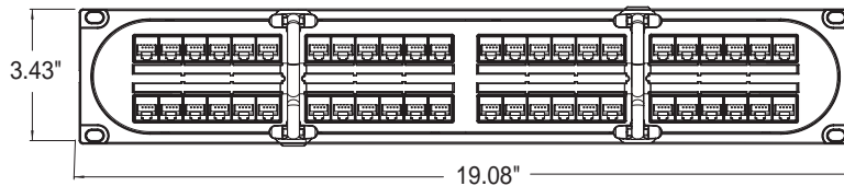
2RU, 48-port 110-style Patch Panel, Cat 6
