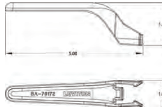
Cable Retainer
