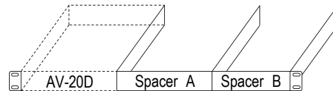
Mounting one AV-20D or AV-60S-AM
