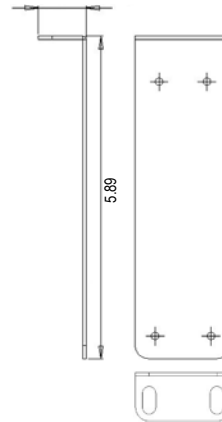
<Ear Bracket> 2pcs included
