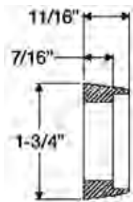
Model CGM Sectional View Showing Dimensions
