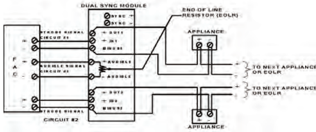
FIG. 1 DUAL CLASS "B" CIRCUIT WITH AUDIBLE SILENCE FEATURE
