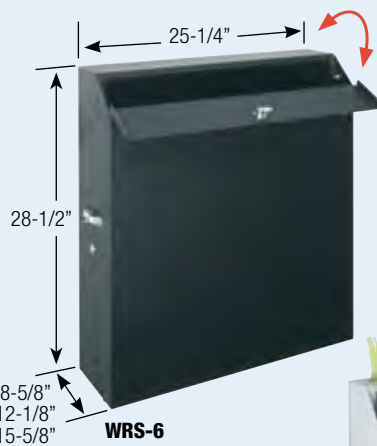
WRP-6 shown in service position
