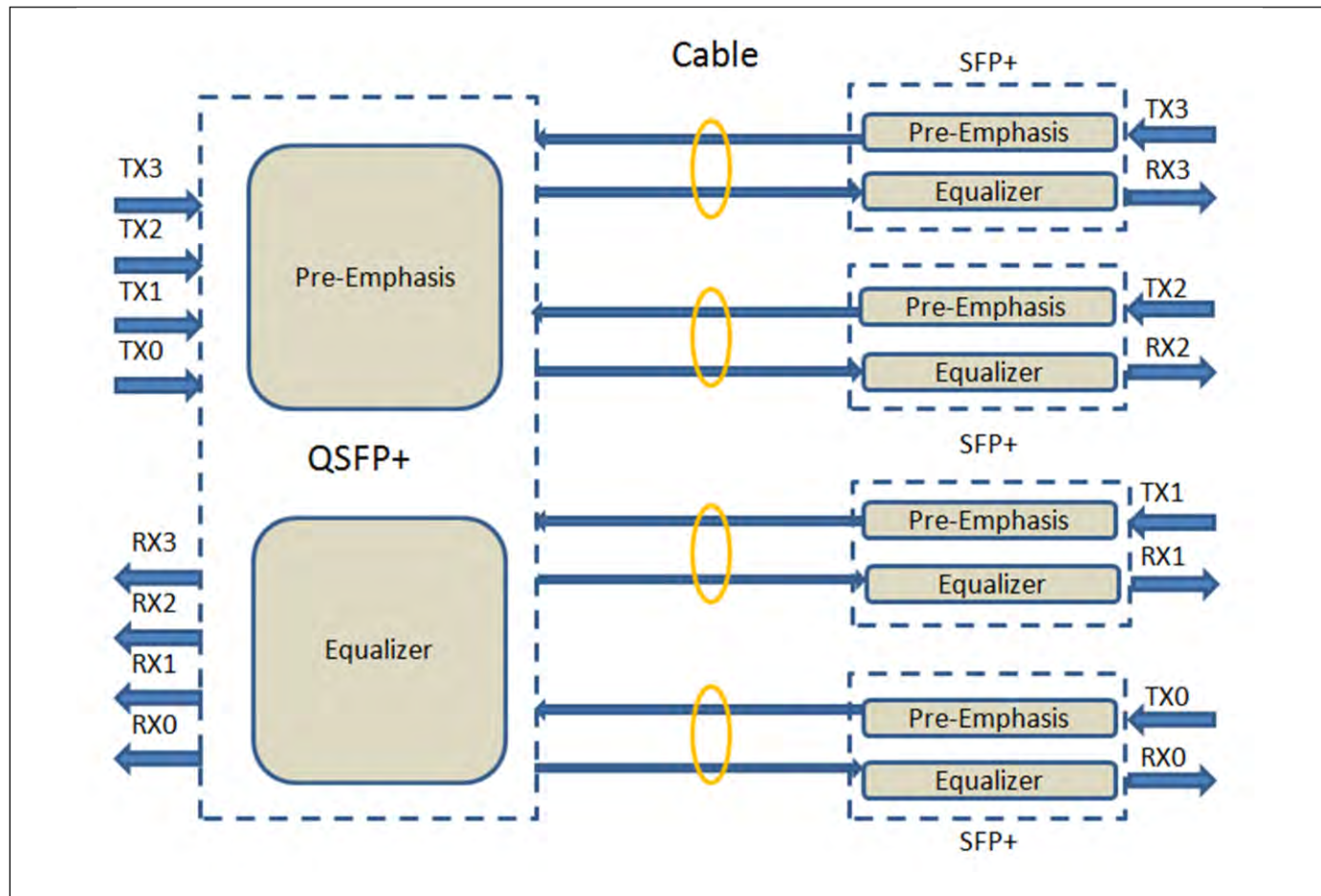
Block Diagram of Transceiver
