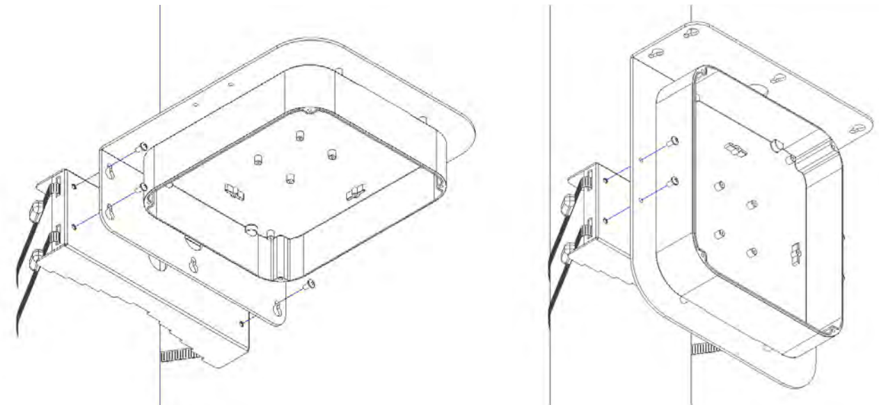
Figure 2 - 1020-RAB Horizontal and Vertical Install
