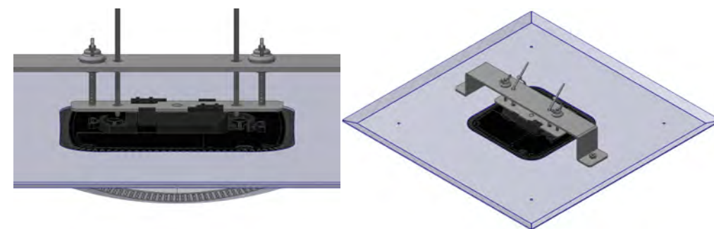
Figure 4 - Attaching Wire Ties
