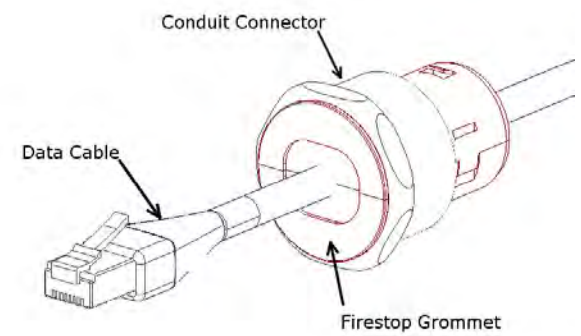
Figure 6 – Firestop Grommet
