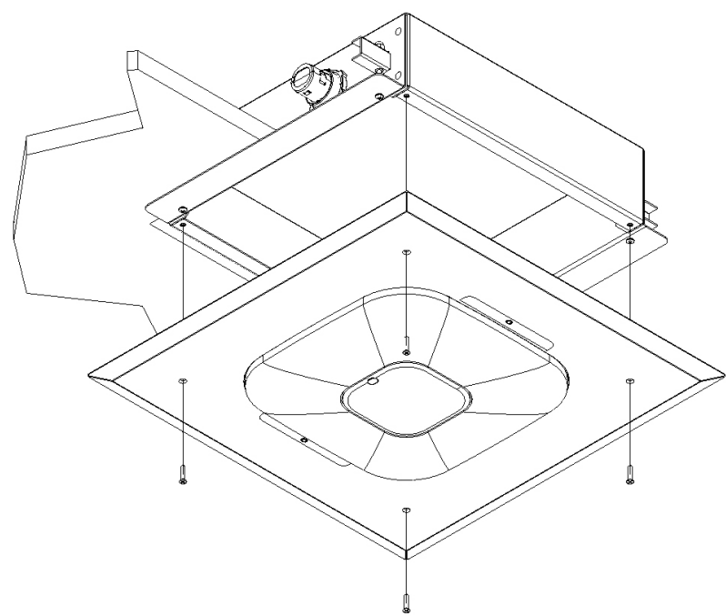
Figure 7 – Trim Install
