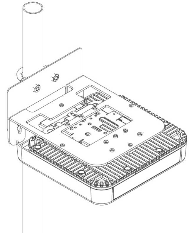
Figure 3 - Completed Installation
