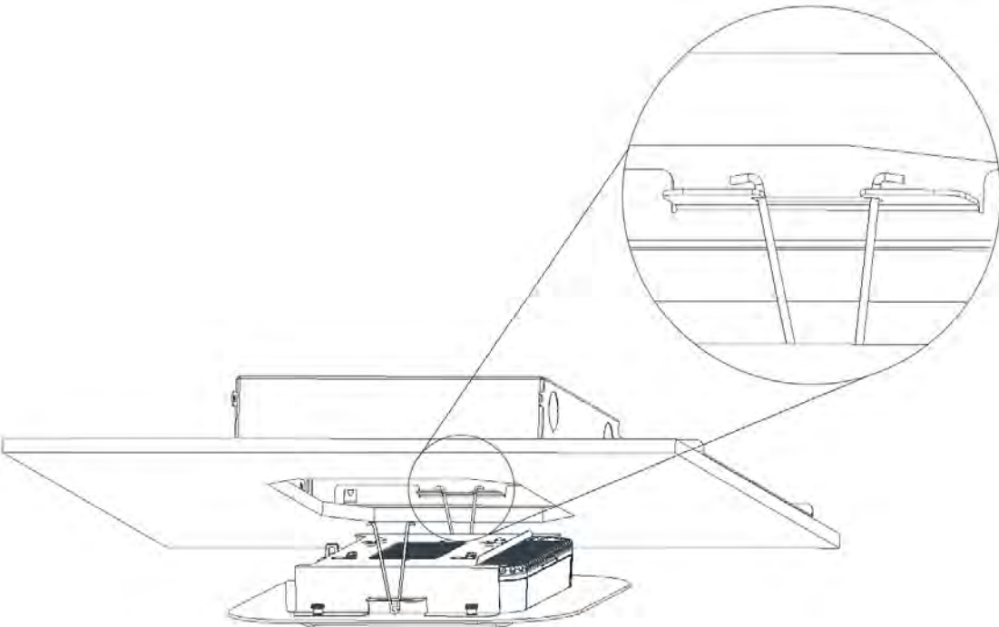
Figure 8 - Assembly of Trim to Backbox
