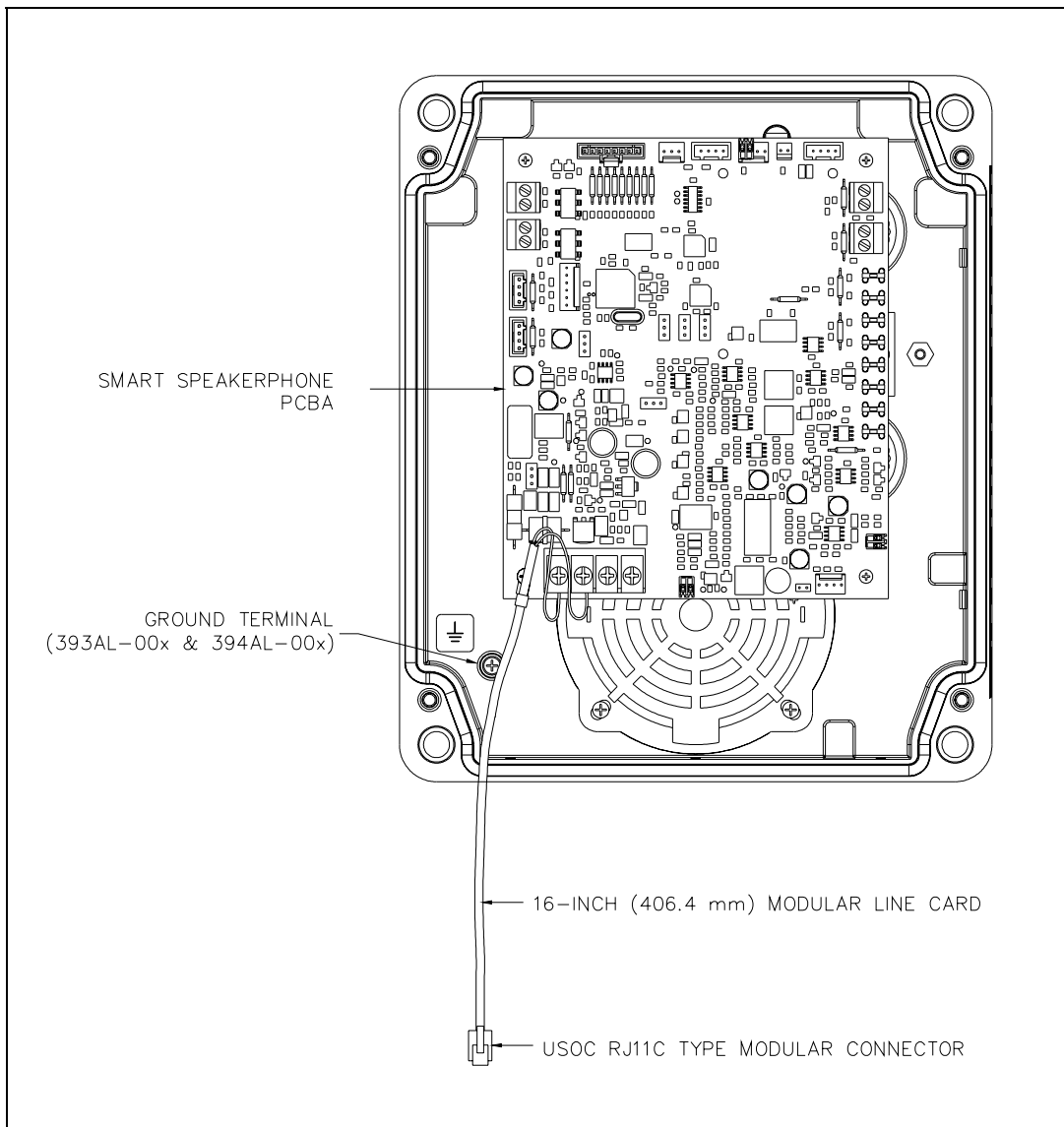
Figure 1. PCBA Connections for Models 393-00x, 393AL-00x, and 394AL-00x
