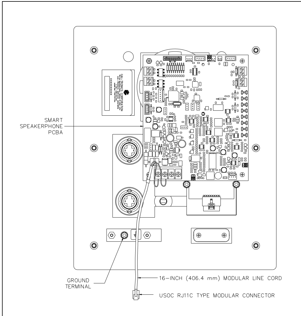
Figure 2. Model 393-00x, 393AL-00x, and 394AL-00x PCBA detail
