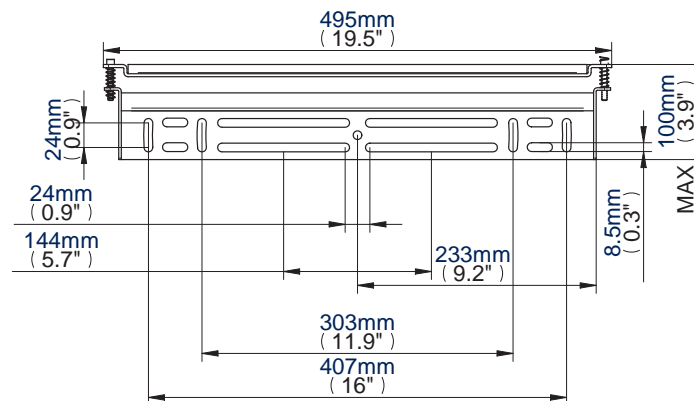
Wall Plate
