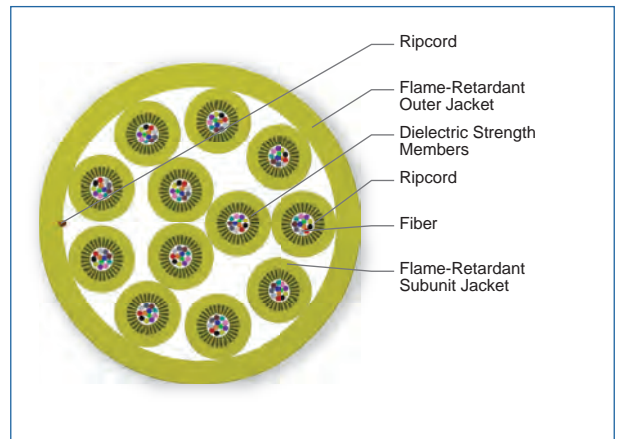
Cross Section of Part Number: 144ED8-T1301-20
