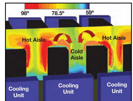
Containment of the hot aisle is a complex problem, even in computer rooms oversupplied with cold air. Belden's AEHC eliminates hot spot issues by providing for a defined hot air return path to the CRAC unit.
