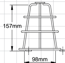
STI 9664 Side View
