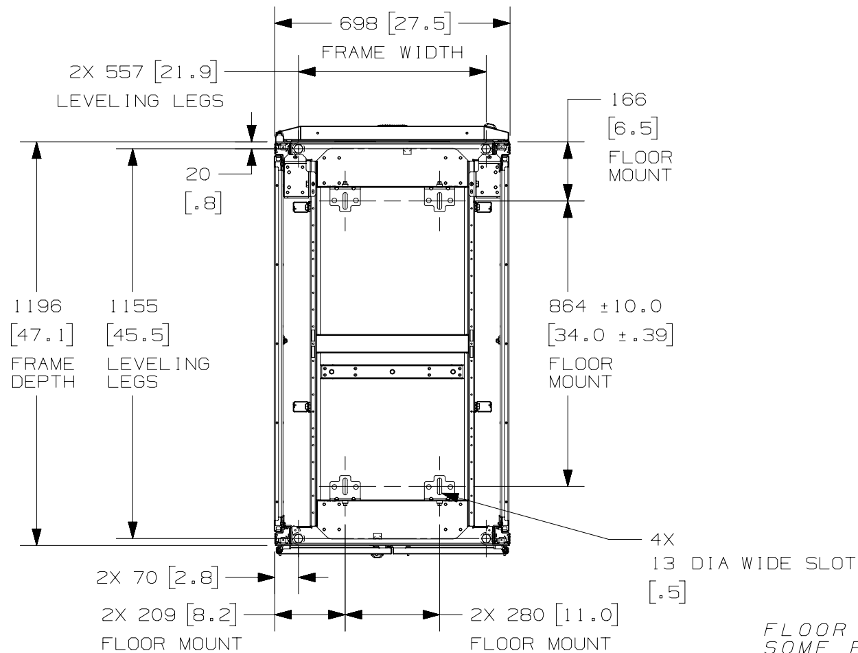
REAR OF CABINET BOTTOM VIEW
