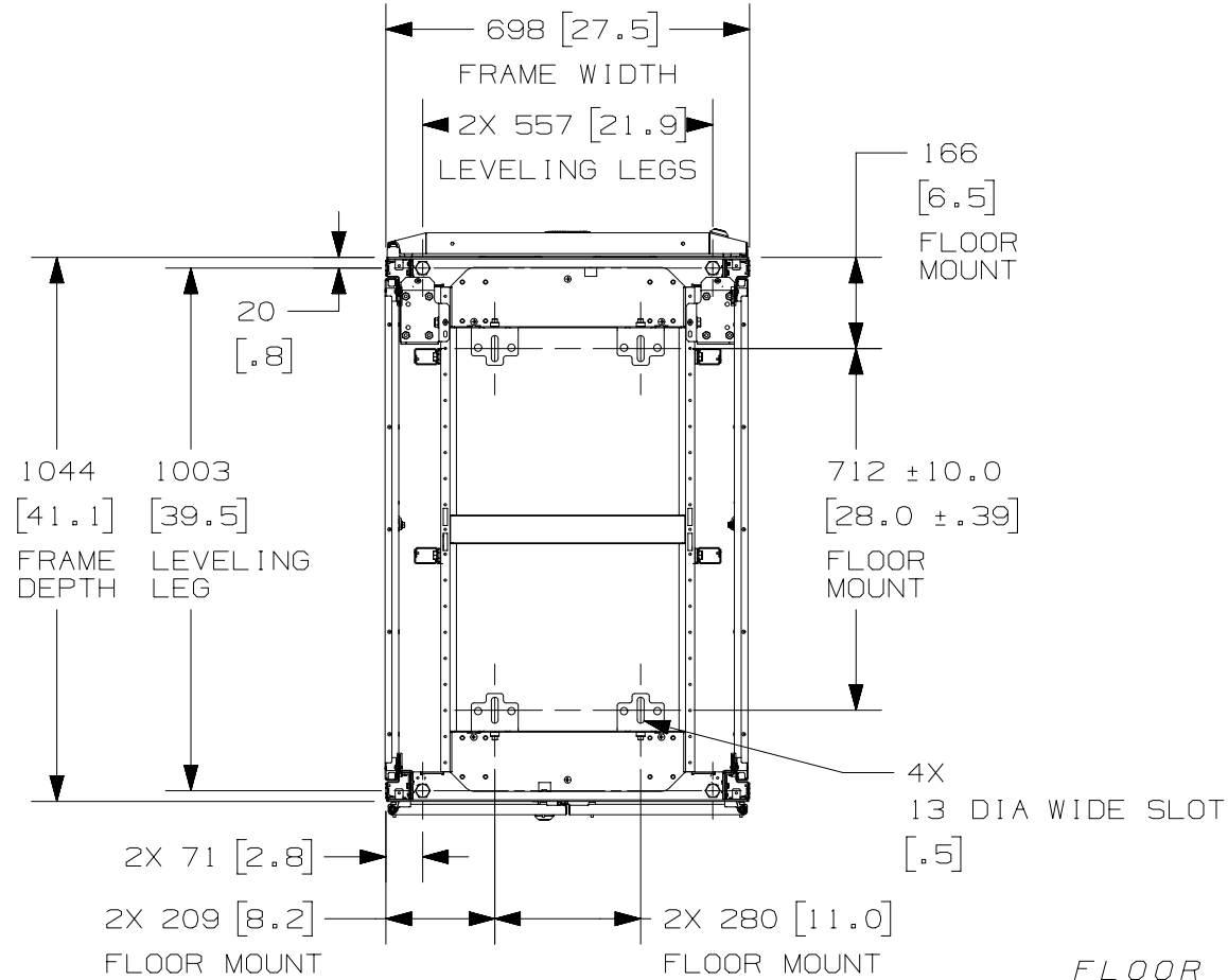
REAR OF CABINET BOTTOM VIEW
