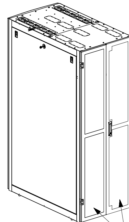
PERFORATED REAR SPLIT DOOR REAR-RIGHT ISO VIEW
