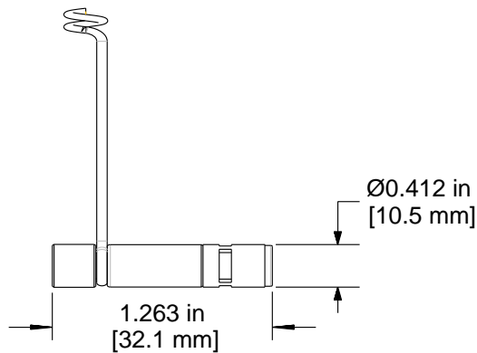
Microphone Dimensions
