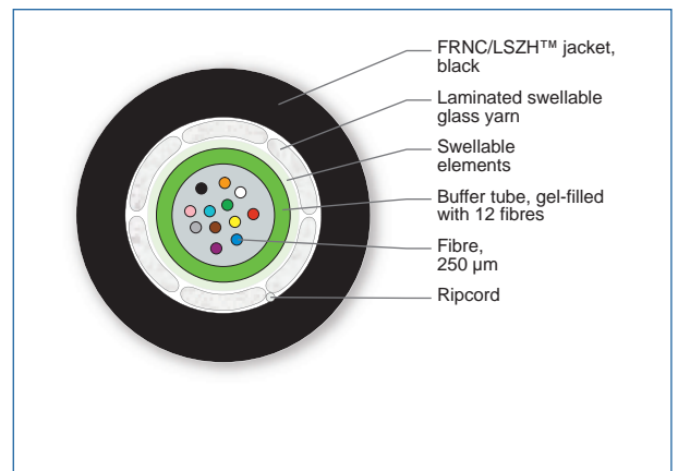
Cross Section of Order Number: 012TEU-13188A2G
