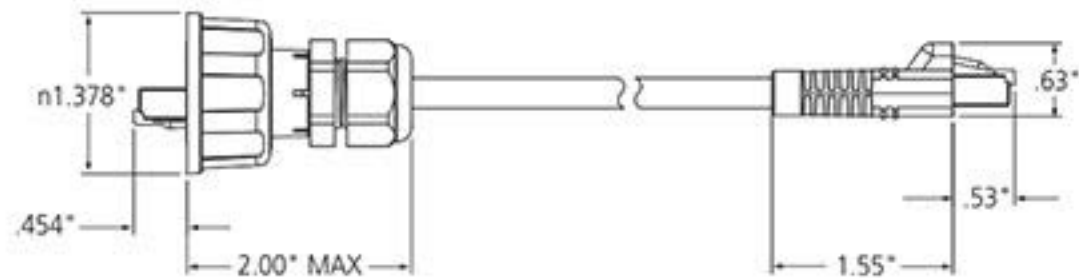
Industrial Plug-to-RJ45 Plug
