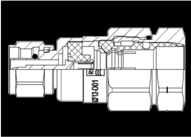
Cut NM-LCF12-D01_DRW.PNG
