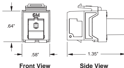
LC QuickPort Adapter
