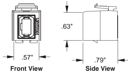
MTP QuickPort® Adapter
