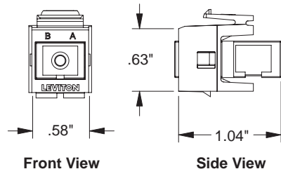
SC/APC QuickPort Adapter
