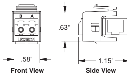
LC QuickPort Adapter
