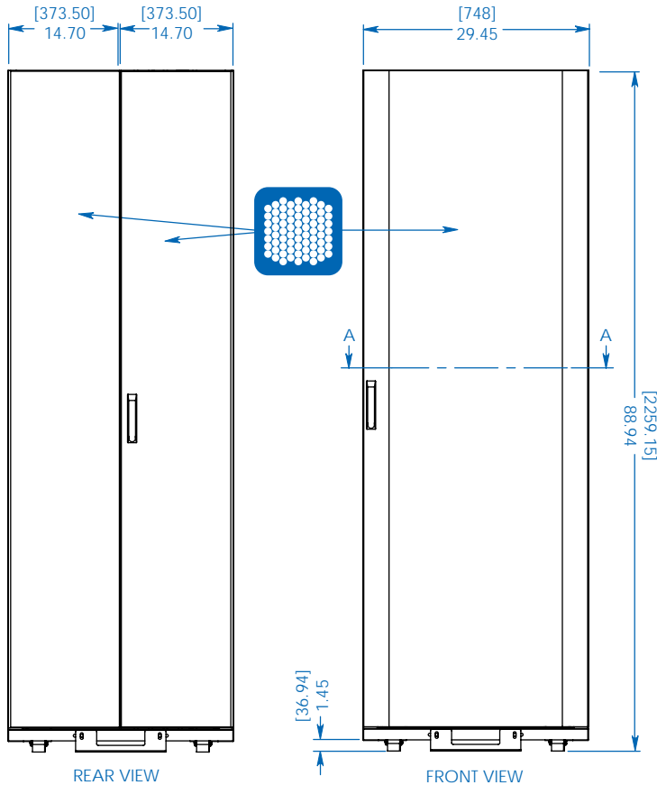
REAR VIEW
