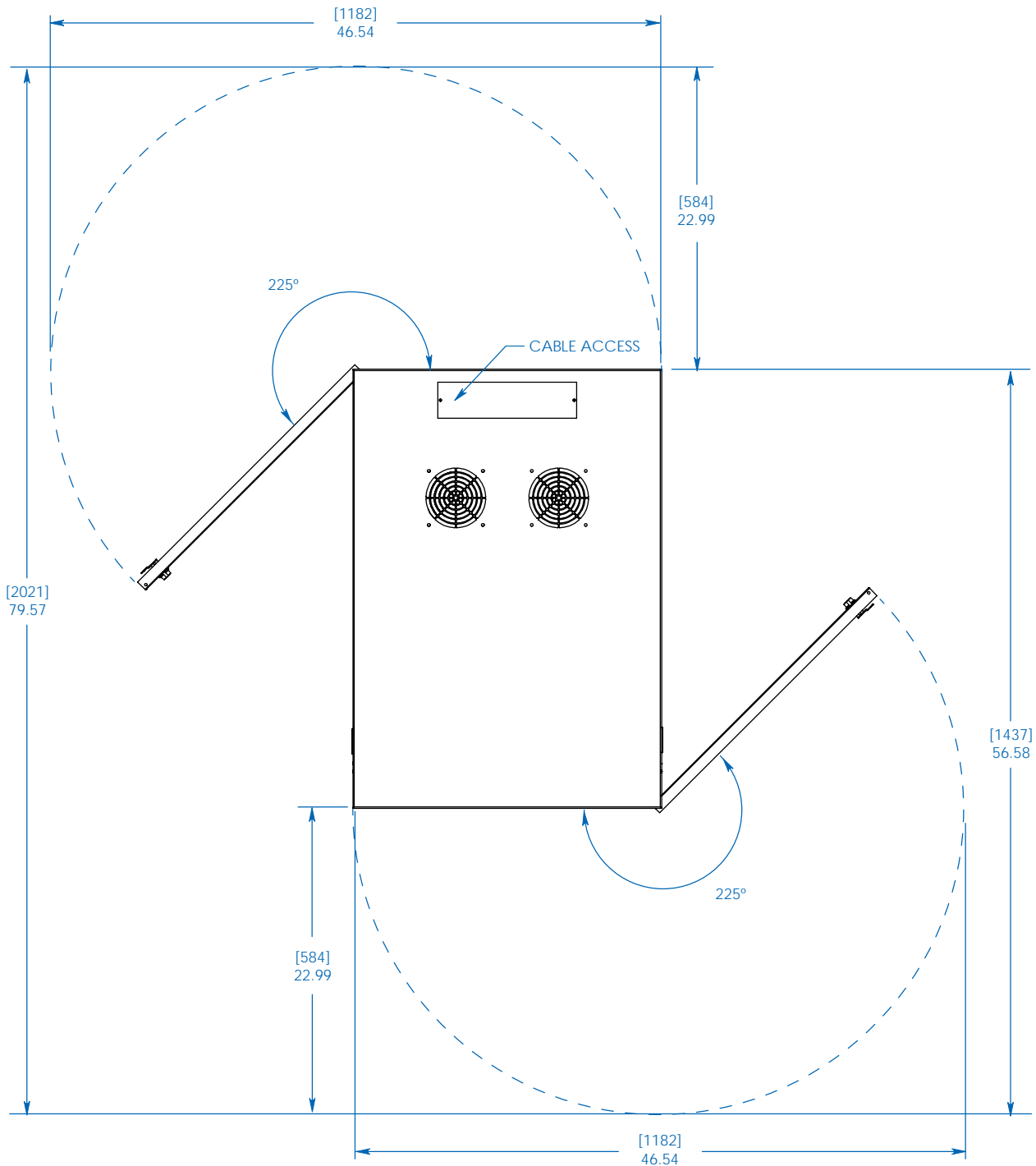
TOP VIEW
