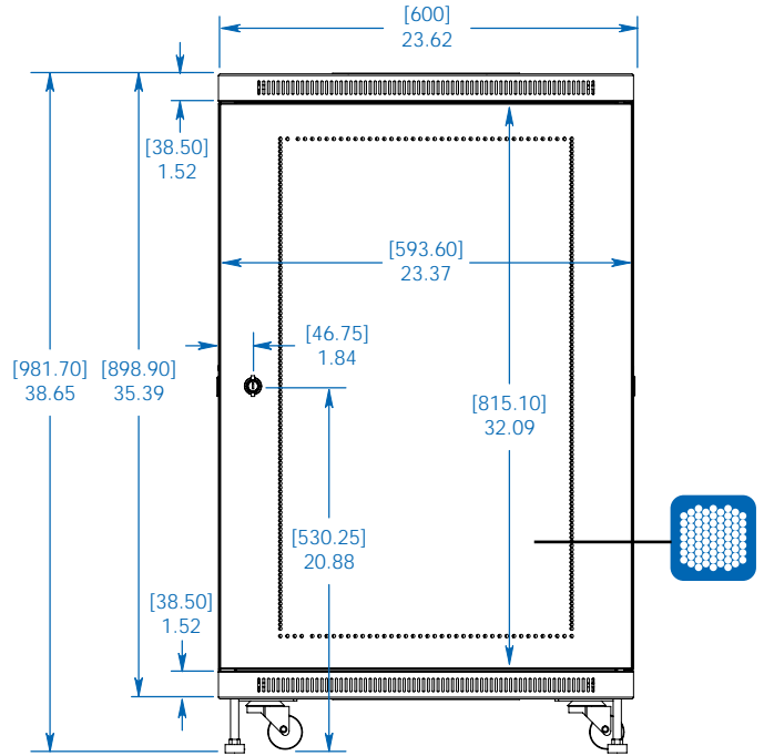
FRONT/REAR VIEW
