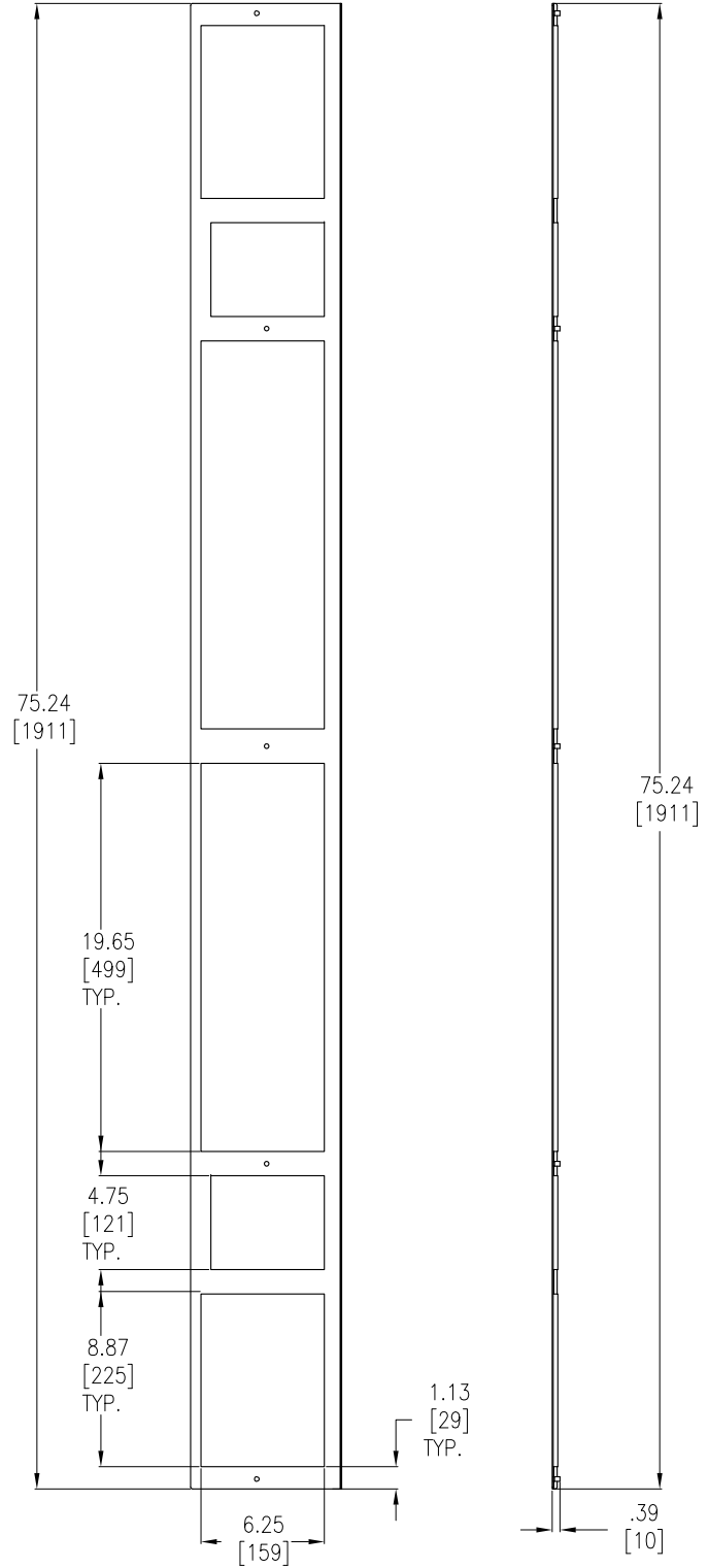
FRONT VIEW
