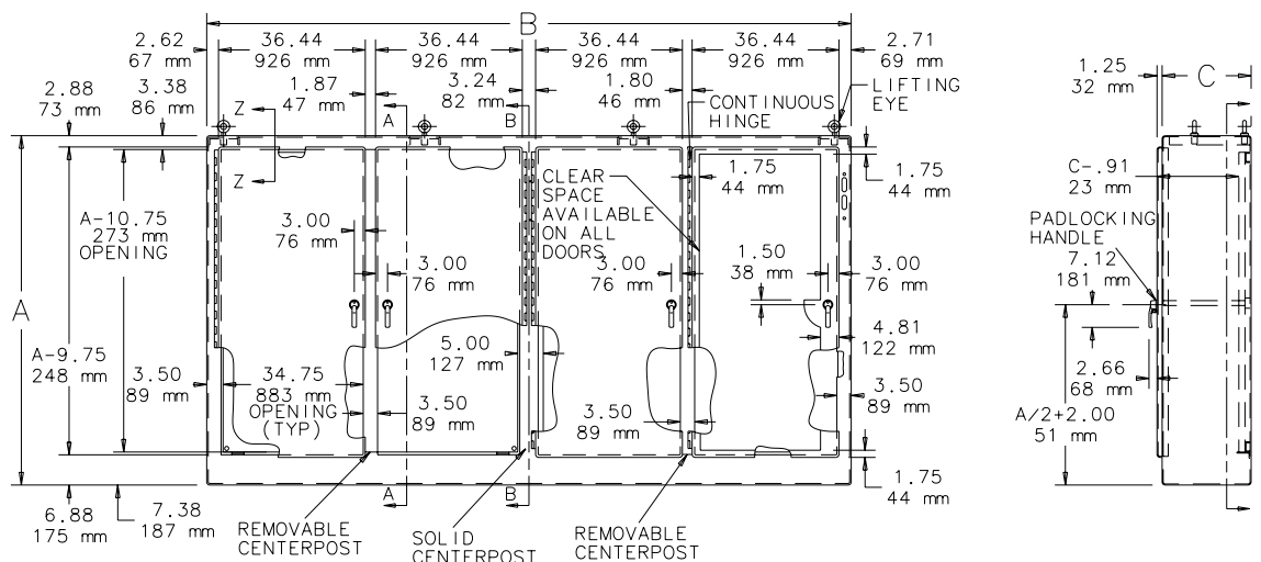
Four-Door Enclosure
