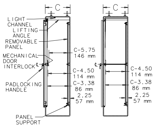
SECTION A-A SECTION B-B
