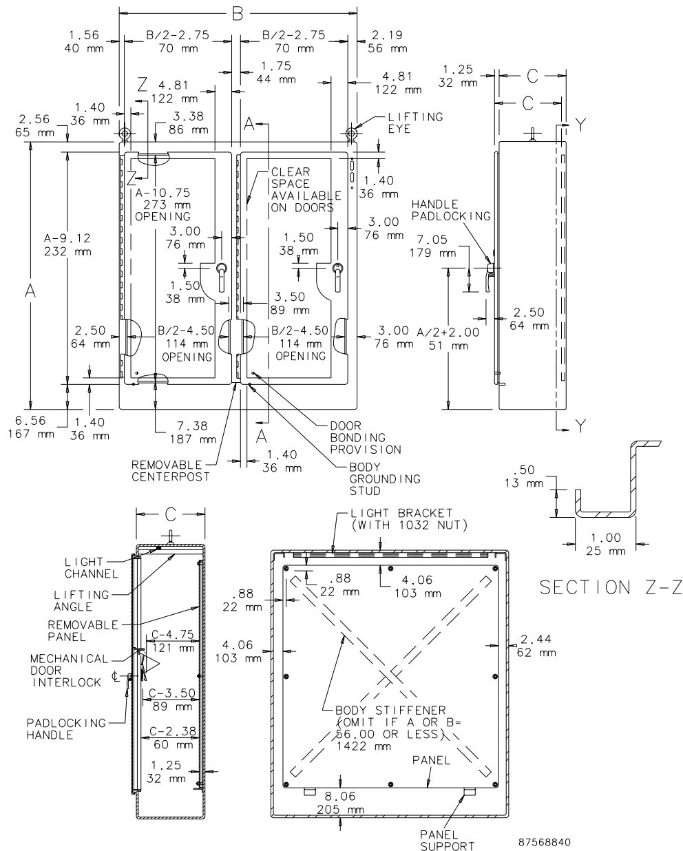
Two-Door Enclosure
