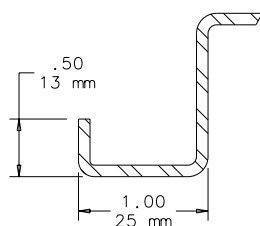
SECTION Z-Z
