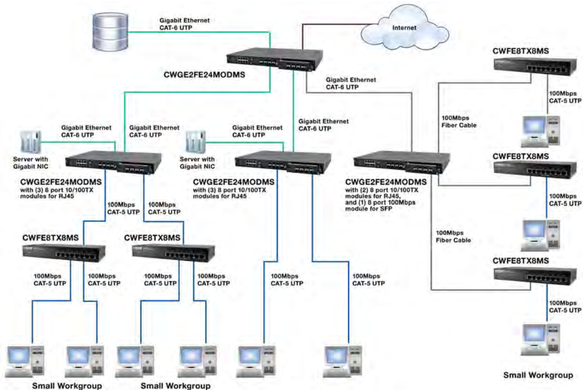
The example of application topology
