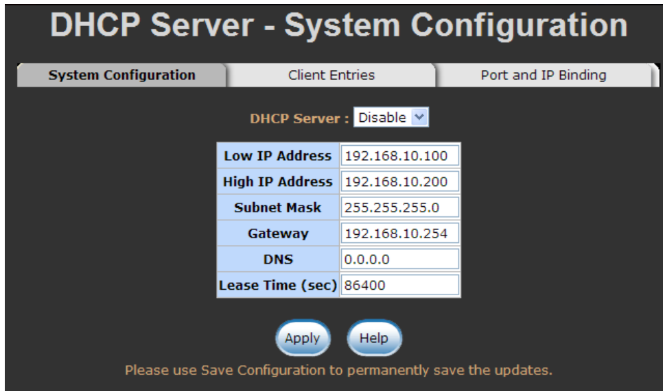
DHCP Server Configuration interface
