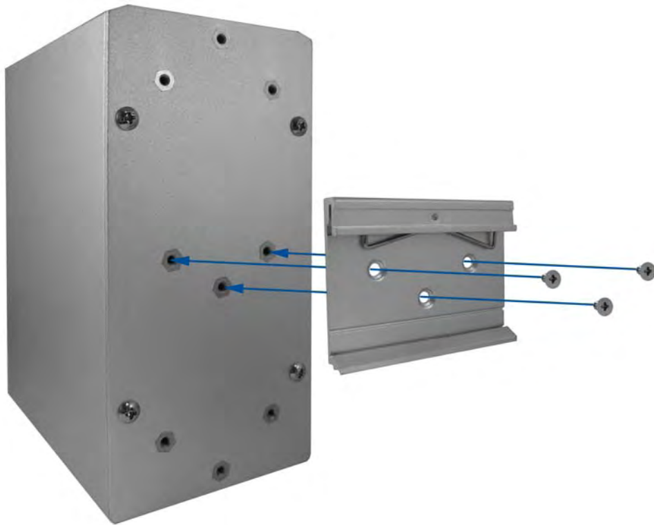
Rear Panel of the switch
