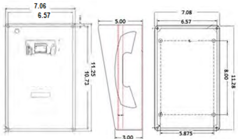
HOB-331/333 HOUSING SPECS
