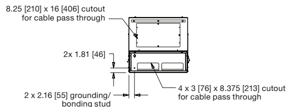
top view backpan and lower wire chamber
