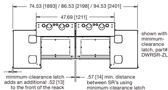
top view open position (with minimum-clearance latch installed)
