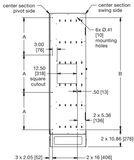
rear view backpan and lower wire chamber
