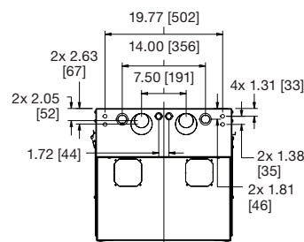
top view knockouts
