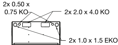
REAR VIEW
