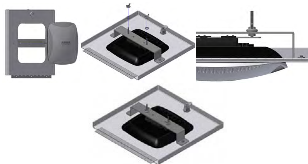
Figure 5 - Fasten T-Bar Bracket.
